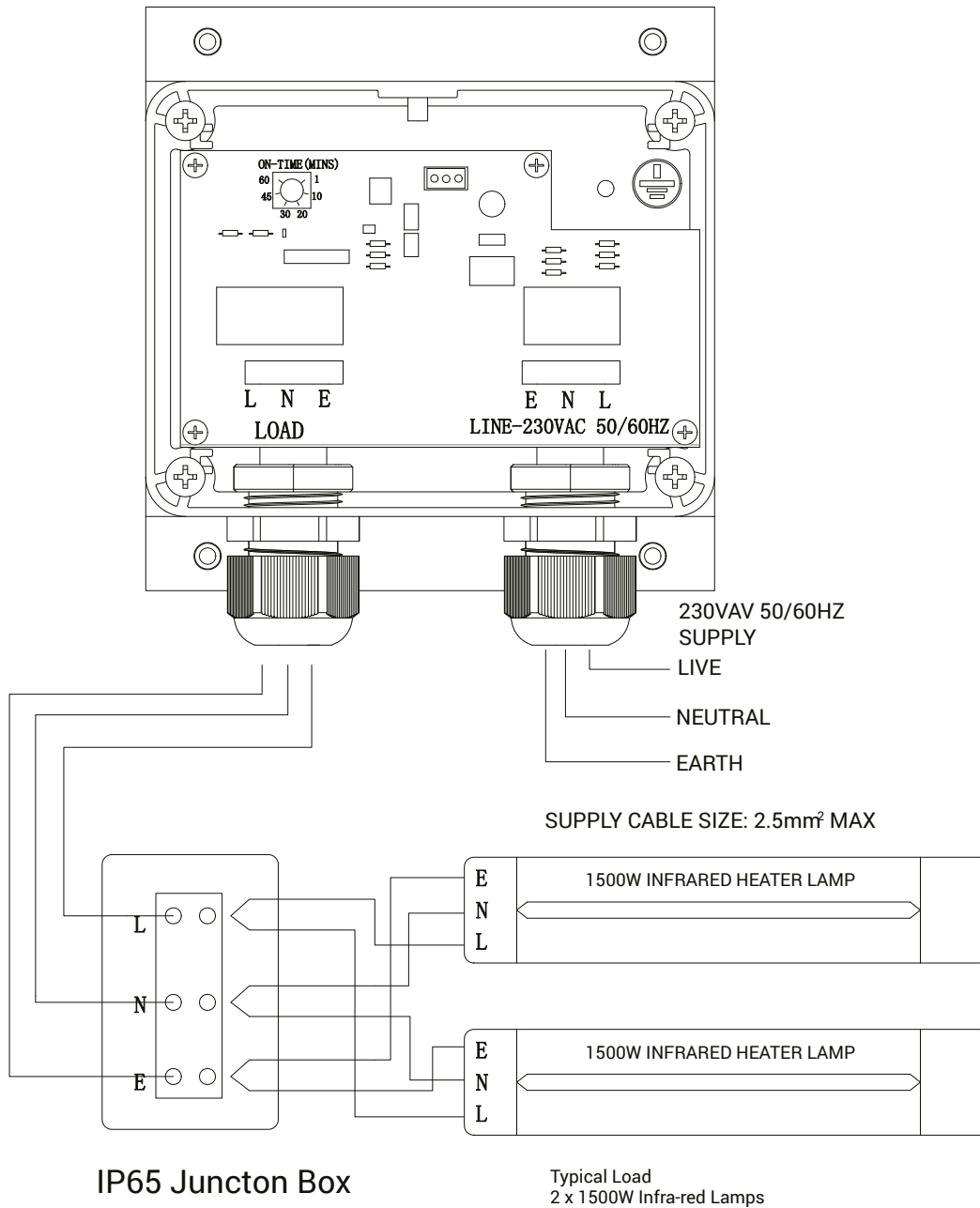
Wiring Diagram
